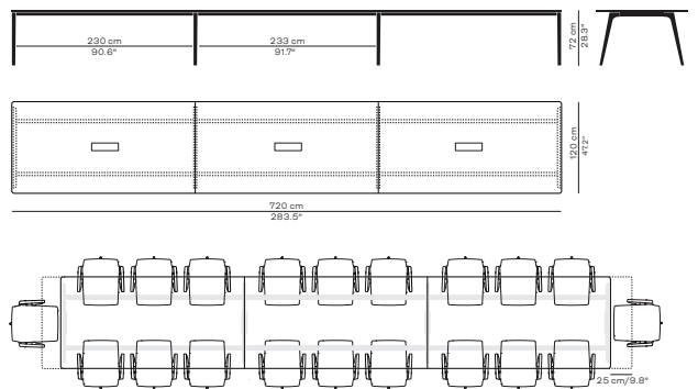
Model: KS425 Three tabletops Available with overhang one- or two end(s) (+25 cm / 9.8") Available widths: 80 cm / 31.5", 90 cm / 35.4", 100 cm / 39.4" or 120 cm / 47.2" Minimum weight: 139 kg / 306 lb
