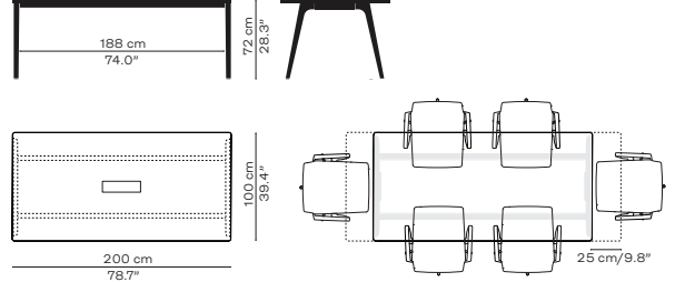
Model: KS421 Single tabletop Available with overhang one- or two end(s) (+25 cm / 9.8") Available widths: 80 cm / 31.5", 90 cm / 35.4" or 100 cm / 39.4" Minimum weight: 46 kg / 101 lb
