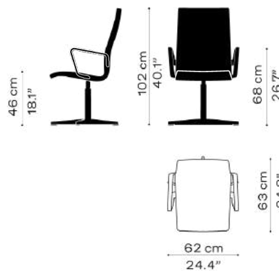
Model: 3273T Medium back 5 Star base Fixed seat height Weight: 11,51 kg / 25.4 Lb
