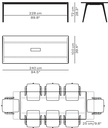
Model: KS422 Single tabletop Available with overhang one- or two end(s) (+25 cm / 9.8") Available widths: 80 cm / 31.5", 90 cm / 35.4", 100 cm / 39.4" or 120 cm / 47.2" Minimum weight: 52 kg / 115 lb
