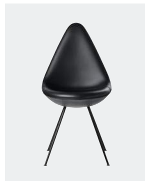
Model: 3110UB Height: 88.5 cm / 34.8 in Seat height: 46 cm / 18.1 in Width: 45.5 cm / 17.9 in Depth: 54.5 cm / 21.5 in
