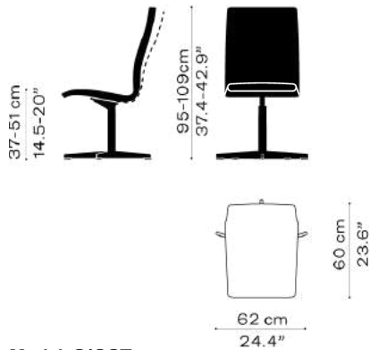
Model: 3193T Medium back 5 Star base Height adjustable Tilting mechanism Weight: 11,35 kg / 25 lb
