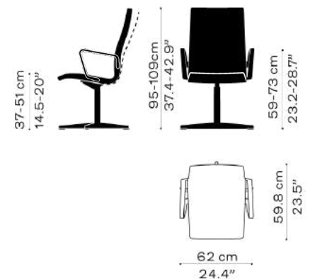
Model: 3293T Medium back 5 Star base Height adjustable Tilting mechanism Weight: 13,64 kg / 30 lb
