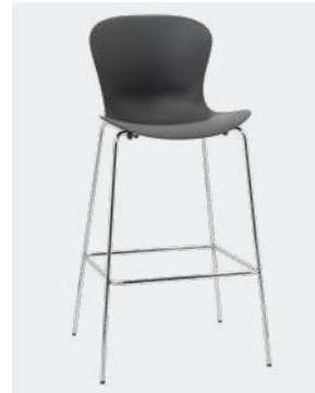
Model: KS59 Height: 109 cm / 43 in Seat height: 76 cm / 30 in Width: 56 cm / 22 in Depth: 54 cm / 21.2 in
