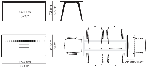
Model: KS420 Single tabletop Available with overhang one- or two end(s) (+25 cm / 9.8") Minimum weight: 41 kg / 90 lbn
