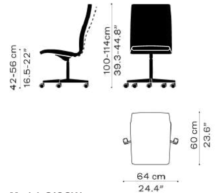
Model: 3193W Medium back 5 Star base on castors Height adjustable Tilting mechanism Weight: 12,05 kg / 26.6 Lb
