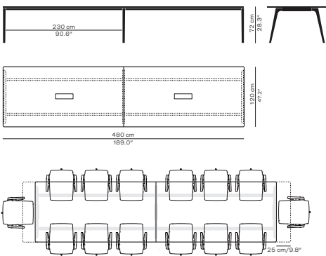
Model: KS424 Two tabletops Available with overhang one- or two end(s) (+25 cm / 9.8") Available widths: 80 cm / 31.5", 90 cm / 35.4", 100 cm / 39.4" or 120 cm / 47.2" Minimum weight: 96 kg / 212 lb
