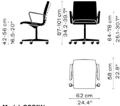
Model: 3291W Low back 5 Star base Height adjustable Tilting mechanism Weight: 8,67 kg / 19 lb
