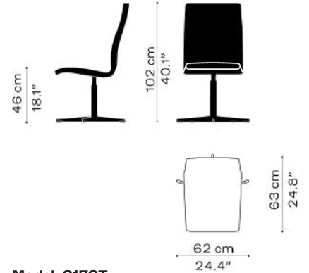
Model: 3173T Medium back 5 Star base Fixed seat height Weight: 9,22 kg / 20.3 Lb
