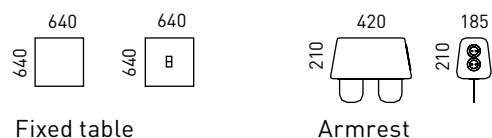
Fixed table
