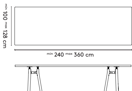
Trestle rectangular 2 connected
